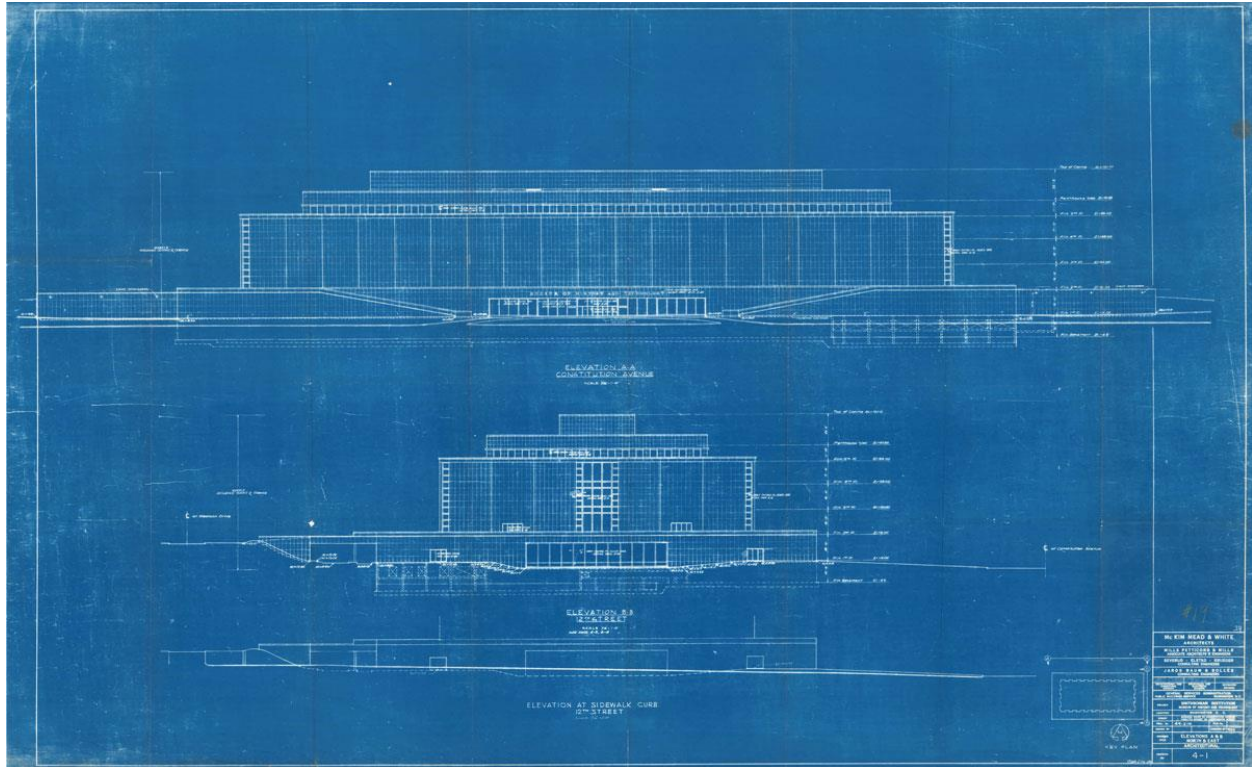
image: Blueprint of Museum of History and Technology, McKim, Mead, and White, architects, elevations of 12th Street and Constitution Avenue sides.
